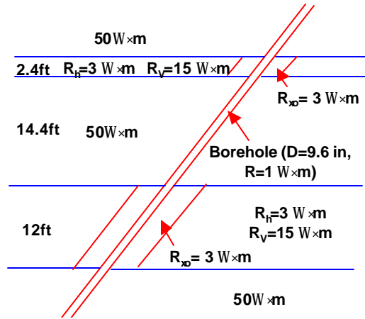
Figure 1. Diagram showing a 5-layer electrical conductivity model and associated geometrical dimensions (not to scale).
