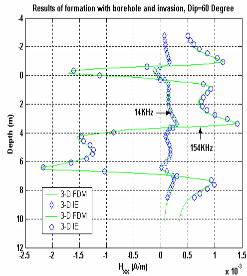
Figure 7. Comparison of the H_{xx} signal simulated with the new algorithm and a 3D-FDM code assuming a 1D formation with borehole and invasion. The borehole has a dip angle of 60^\circ . Results for 14KHz and 154KHz are shown on this figure.
