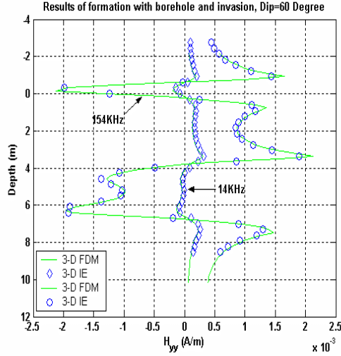
Figure 8. Comparison of the H_{yy} signal simulated with the new algorithm and a 3D-FDM code assuming a 1D formation with borehole and invasion. The borehole has a dip angle of 60^\circ . Results for 14KHz and 154KHz are shown on this figure
