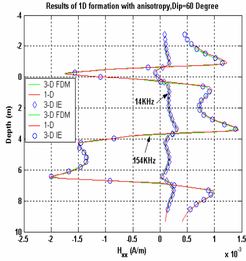
Figure 4. Comparison of the H_{xx} signal simulated with the new algorithm and a 1D code assuming a 1D formation. The tool and the formation form an angle of 60^\circ . Results for 14KHz and 154KHz are shown on this figure.
