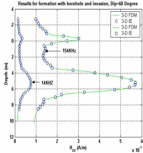
Figure 6. Comparison of the H_{zz} signal simulated with the new algorithm and a 3D-FDM code assuming a 1D formation with borehole and invasion. The borehole has a dip angle of 60^\circ . Results for 14KHz and 154KHz are shown on this figure.
