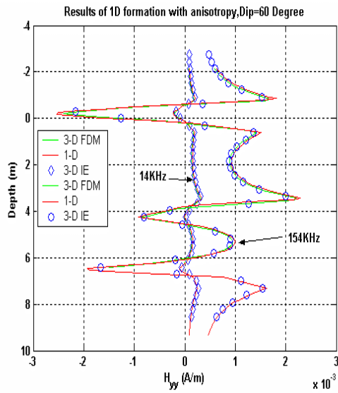
Figure 5. Comparison of the H_{yy} signal simulated with the new algorithm and a 1D code assuming a 1D formation. The tool and the formation form an angle of 60^\circ . Results for 14KHz and 154KHz are shown on this figure.
