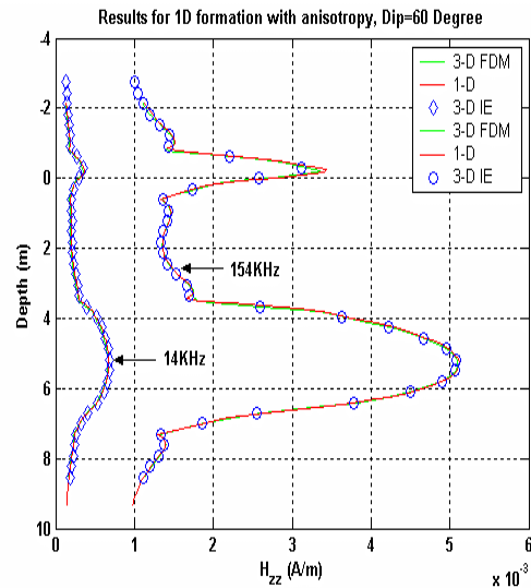
Figure 3. Comparison of the H_{zz} signal simulated with the new algorithm and a 1D code assuming a 1D formation. The tool and the formation form an angle of 60^\circ . Results for 14KHz and 154KHz are shown on this figure.
